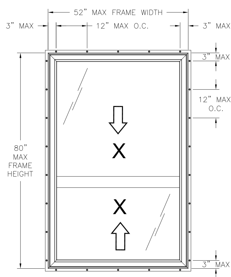
S-SERIES DOUBLE HUNG EXTERIOR VIEW FIN INSTALLATION
