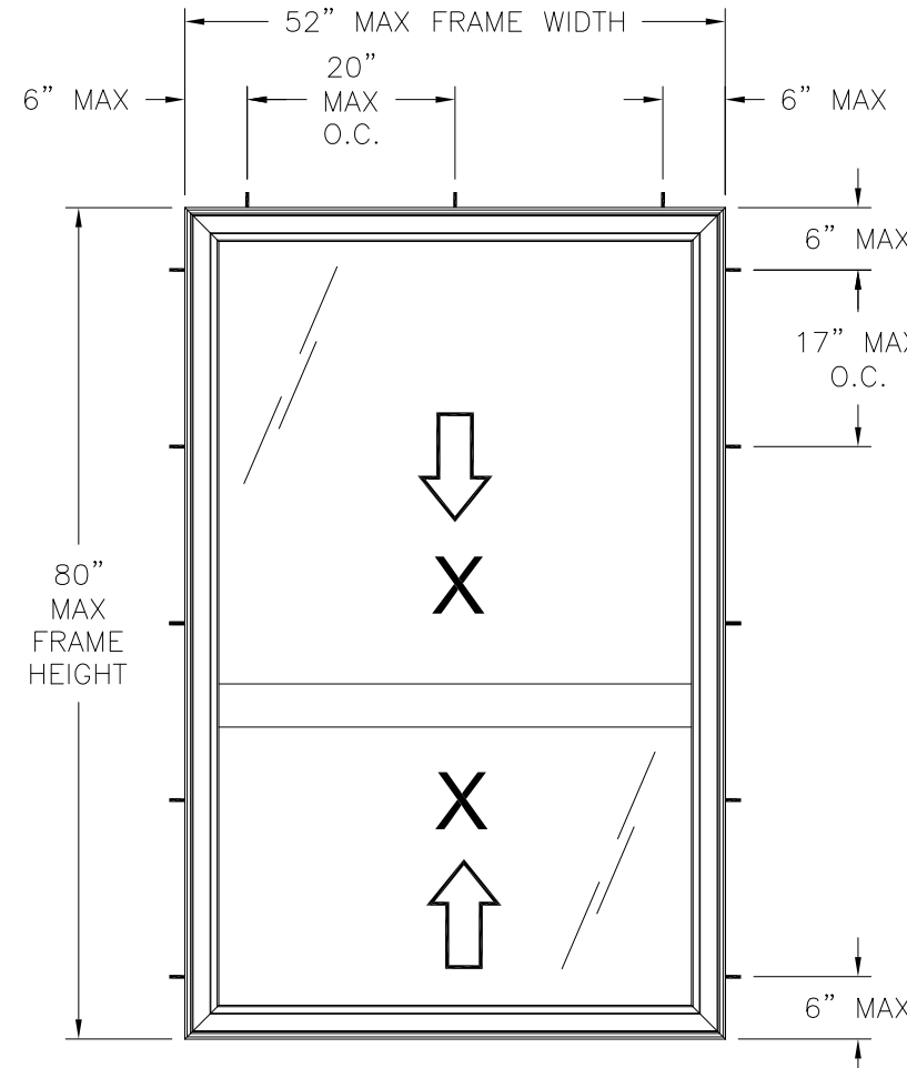
CAMBRIDGE DOUBLE HUNG EXTERIOR VIEW FRAME INSTALLATION
